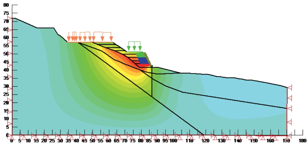
Figure 5: Vertical displacements for scenarios 2 (engineered slope with piles L=18 m, D=0.6 m).
