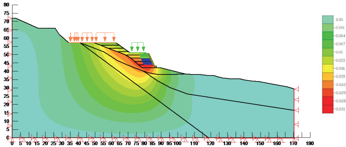
Figure 4: Vertical displacements for scenario 1 (unreinforced base slope)
